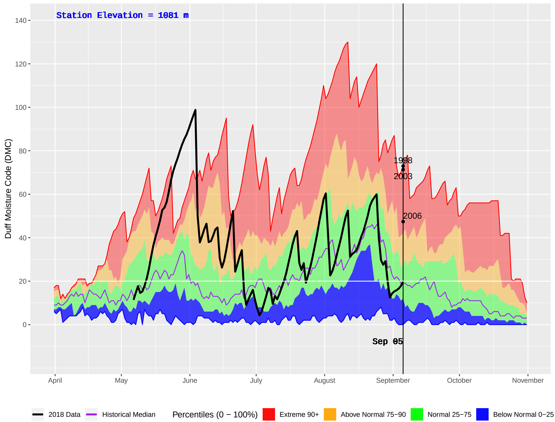
GAVIN (227) : Historical (1981–2016) and Current (2018) Daily Duff Moisture Code (DMC)
